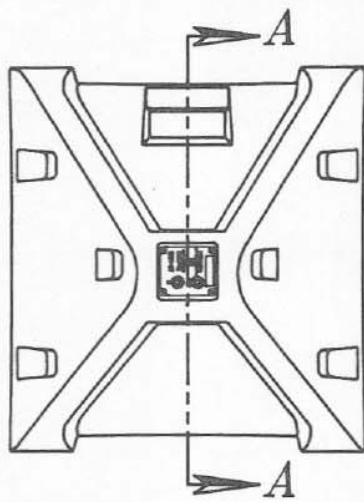
BACK VIEW: 1/2 SCALE (ORIENTATION OF INPUT PANEL)
